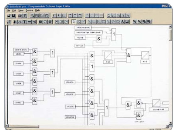
Programmable scheme logic editor (MiCOM S1 Studio)
